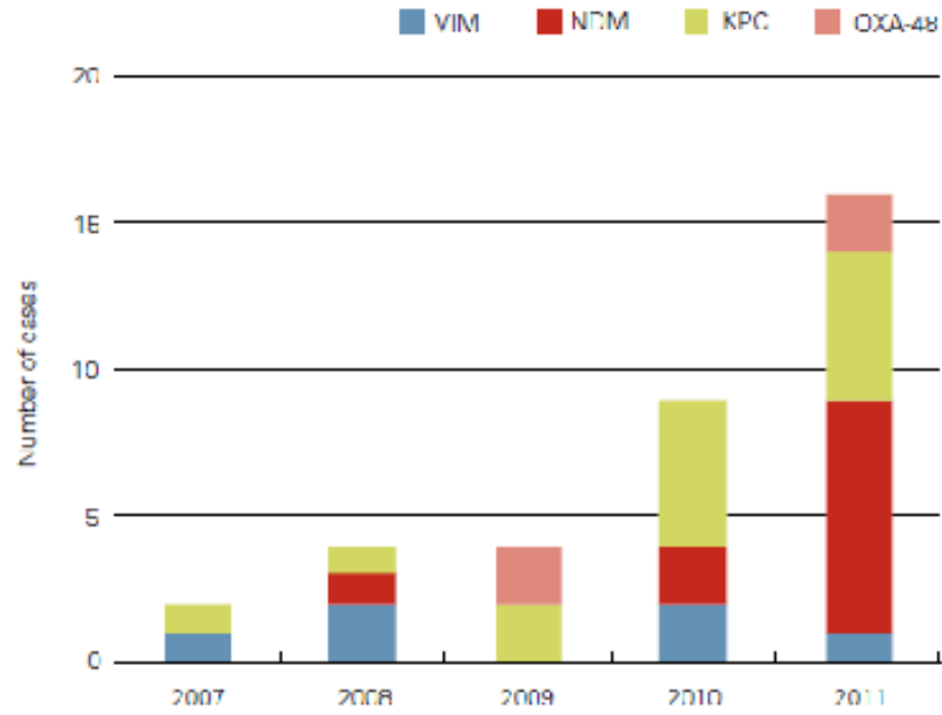
FIGURE 4.13. Numbers and types of ESBL CARB in Enterobacteriaceae in Sweden 2007-2011.
