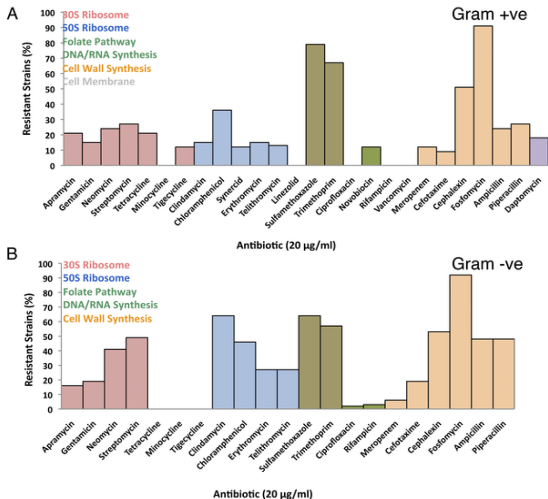
Figure 2. Resistance levels of Lechuguilla cave bacteria at 20 \mu g/ml against various antibiotics: (top) Gram-positive strains (bottom) Gram-negative strains.
